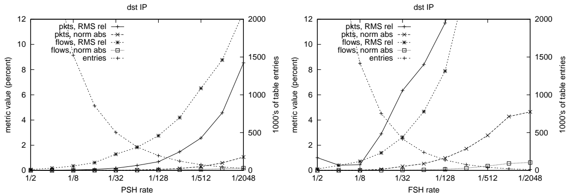
Figure 3: Trading memory for accuracy with sample-and-hold rates. Counting done on Backbone with DDoS with tuple set algorithm.
