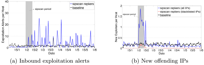
Fig. 2. Daily number of inbound exploitation alerts and new offending IPs per target host over a period of 5 months. The shaded region marks the duration of the sipskan.
