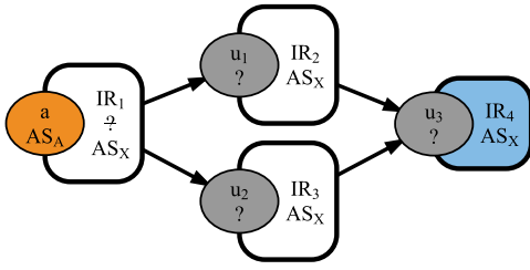
Figure 8: Annotating IRs with unannounced interface addresses. IR_4 was annotated by the last hop heuristic. In the first iteration of the graph refinement loop IR_2 and IR_3 are annotated with AS_X , enabling the annotation of IR_1 .
