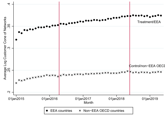
Fig. 9. Average log customer cone of networks in EEA and non-EEA OECD countries. Notes: The dots represent \overline{\log(NtwrkCustCone_{k \in EEA,t})} , the log customer cone averaged among networks owned by EEA countries. The crosses represent \overline{\log(NtwrkCustCone_{k \in OECD \setminus k \in EEA,t})} , the log customer cone averaged among networks owned by non-EEA OECD countries. Non-EEA and non-OECD countries’ networks are not included in taking the averages. Only networks present throughout Jan 2015 – June 2019 are used to take the averages. Regression including month and network fixed effects has the coefficient on POST_e \times EEA = -.007^* ( se = 0.004 , clustered by country) and the coefficient on POST_a \times EEA = 0.011^{***} ( se = 0.004 , clustered by country). Though both are significantly different from zero, their magnitudes are economically small.
