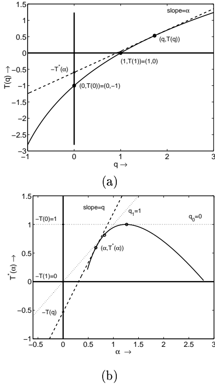
Figure 6: The Legendre transform T \mapsto T^* in the simple case of a concave, differentiable function such as the spectrum of a \beta MWM ((66) with p = 1.66 , H = 0.85 ). Set \alpha = T'(q) ; then T^*(\alpha) is such that the tangent at (q, T(q)) passes through (0, -T^*(\alpha)) . In other words, -T^*(\alpha) + q\alpha = T(q) (see (51)). By symmetry, the tangent at (\alpha, T^*(\alpha)) has slope q and passes through (0, -T(q)) . There are two special values of q . Trivially, T(0) = -1 , hence the maximum of T^* is 1. In addition, every positive increment process has T(1) = 0 , hence T^* touches the bisector.
