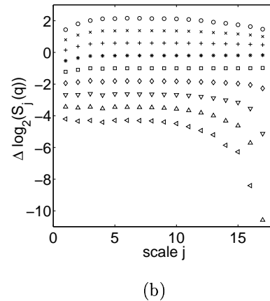
Figure 10: (a) Log-log moment scaling and (b) incremental scaling for the \beta MWM synthesized data. (See Figure 8 for more description.) The synthetic data exhibits a linear multifractal scaling, with the exception of strongly negative q 's and large j .
