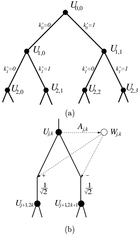
Figure 3: (a) More detailed tree structure of scaling coefficients. (b) MWM construction: At scale j , we form the wavelet coefficient as the product W_{j,k} = A_{j,k}U_{j,k} , with A_{j,k} a random variable distributed in [-1, 1] . Then, at scale j + 1 , we form the scaling coefficients U_{j+1,2k} and U_{j+1,2k+1} as sums and differences of U_{j,k} and W_{j,k} (normalized by 1/\sqrt{2} ).
