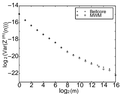
Figure 7: Variance-time plot of the Bellcore pAug data “x” and one realization of the \beta MWM synthesis “o”. Here m denotes the level of aggregation and Z^{(m)}(n) , the aggregated process defined through (11).
