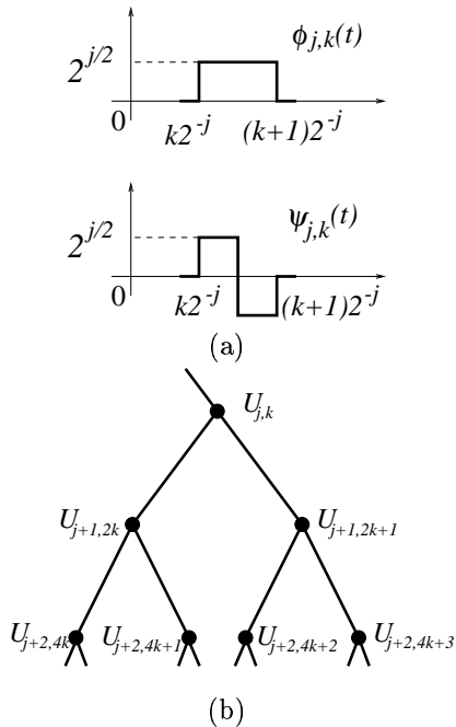
Figure 1: (a) The Haar scaling and wavelet functions \phi_{j,k}(t) and \psi_{j,k}(t) . (b) Binary tree of scaling coefficients from coarse to fine scales.
