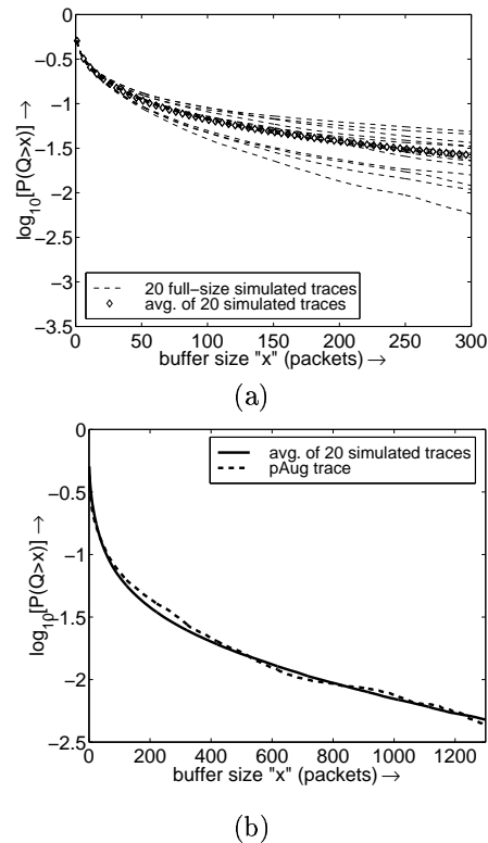
Figure 12: Comparison of the queuing behavior of pAug with 20 full-size synthesized traces. Displayed are the tail probabilities of buffer occupancy vs. buffer size. In (a) observe the variability of the queue performance of the synthesized traces. In (b) observe that the average queue performance of simulated traces and that of the real trace match closely.
