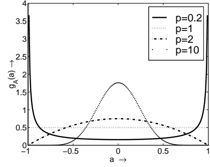
Figure 4: Examples of the pliable pdf g_A(a) of the \beta(p, p) random variable A , for different values of p . For p = 0.2 , A resembles a binomial random variable, and for p = 1 it has a uniform density. For p > 1 the density resembles a truncated Gaussian density, with the resemblance increasing with p .
