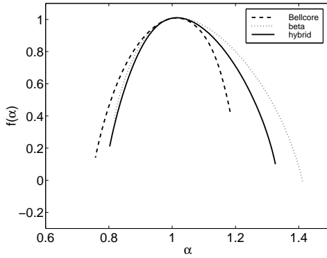
Figure 9: Multifractal spectra (51) of the Bellcore pAug data, \beta MWM synthesis, and a hybrid MWM employing beta distributions at coarse scales and point masses at fine scales. The spectra were obtained through the Legendre transform of the scaling of the moments (see Figures 8 and 10). The close match in the upper left part, which corresponds to q values (=slopes of tangents to the spectrum) between 0 and 2, indicates that the \beta MWM matches these low ( q th) order moments very well. The divergence of the spectra on the right indicates that the chance of observing large \alpha in the \beta MWM data is somewhat too high. This behavior is improved significantly by adding point mass multipliers in the fine scales.
