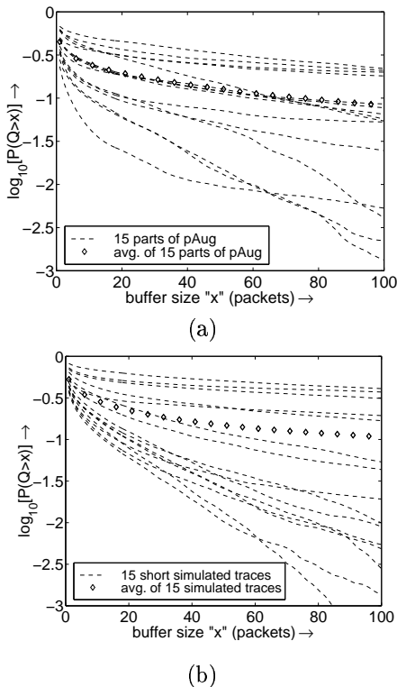
Figure 11: Here we partition the pAug trace into 15 sub-traces of equal number of packets and compare their queuing behavior with that of 15 synthesized traces of the same length. In (a), observe that the real sub-traces have a wide variation in tail queue behavior. In (b), observe that the synthesized traces display a similar variation in tail queue behavior.
