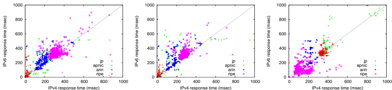
Figure 1: Distribution of IPv6/IPv4 RTT from WIDE (left), IIJ (middle), and ES (right)
